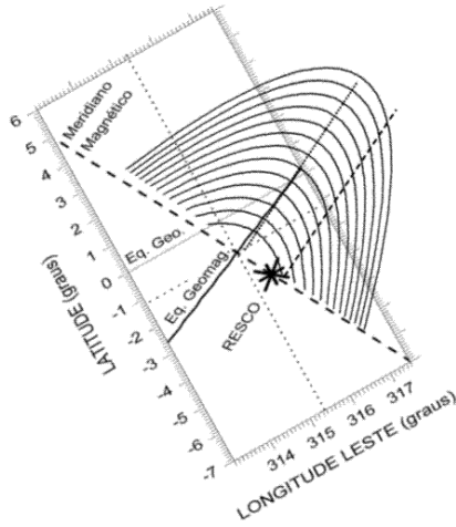
Fig. 1. Sketch of the magnetic field lines (between 89 and 125 km) on the magnetic meridian corresponding to the magnetic longitude of São Luís.
