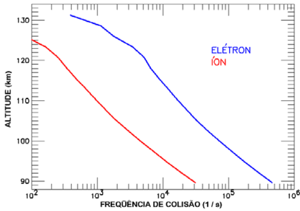
Fig. 3. Vertical profile of the ion-neutral collision rate (red line) and vertical profile of the electron-neutral collision rate (blue line) calculated for the RESCO radar site location, covering the range height from 90 to 130 km, during equinox, at 12 h (local time).
