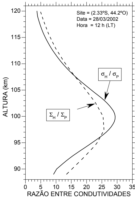
Fig. 5. Vertical profiles of the local Hall-to-Pedersen conductivity ratio calculated using local conductivities (continuous line) and magnetic field lines integrated conductivities (dashed line).
